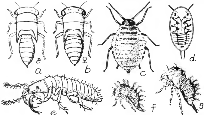
Fig. 70 a & b, Idiocerus provancheri Van D.; c, Aphid; d, Aleyrodes sp., e, Magicicada septendecim (L.); f & g, Two different instars of Stictocephala sp. (U.S.D.A.)
